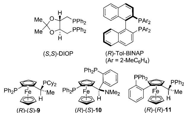
Figure 1. Structures of chiral bidentate phosphane ligands.
