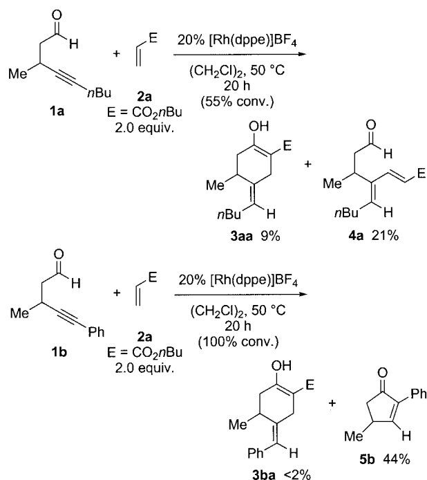
Scheme 3. Rhodium-catalyzed [4+2] carbocyclization of 5-alkyl- and 5-phenyl-4-pentynals with butyl acrylate.
