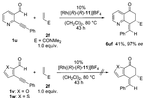
Scheme 11. Rhodium-catalyzed regio- and enantioselective [4+2] carbocyclization of heterocyclic 4-alkynals with N,N -dimethylacrylamide.
