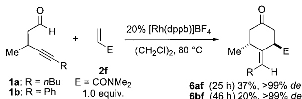
Scheme 6. Rhodium-catalyzed regio- and diastereoselective [4+2] carbocyclization of 5-butyl- and 5-phenyl-3-methyl-4-pentynals with N,N -dimethylacrylamide.
