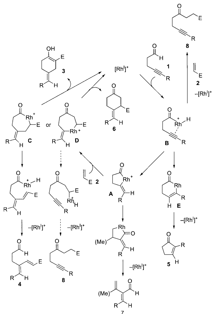
Scheme 12. Possible mechanism for rhodium-catalyzed intermolecular [4+2] carbocyclization of 4-alkynals with electron-deficient alkenes.
