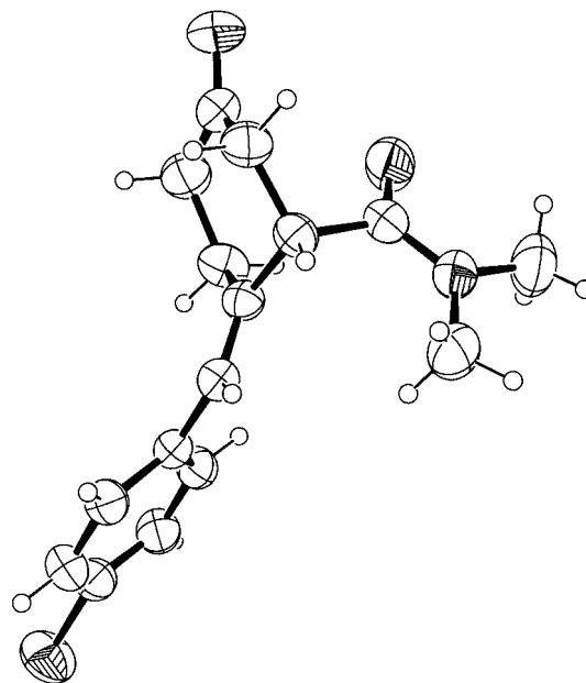
Figure 2. ORTEP diagram of (S)-(+)- 6kf . Ellipsoids drawn at the 50% probability level.
