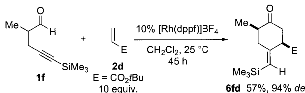
Scheme 4. Rhodium-catalyzed regio- and diastereoselective [4+2] carbocyclization of 2-methyl-5-trimethylsilyl-4-pentynal with tert -butyl acrylate.
