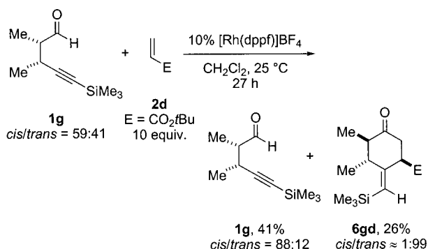
Scheme 5. Rhodium-catalyzed diastereoselective kinetic resolution of 2,3-dimethyl-5-trimethylsilyl-4-pentynal.
