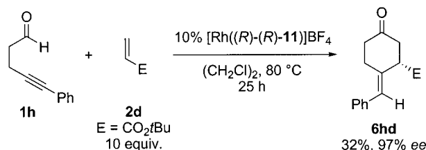
Scheme 8. Rhodium-catalyzed regio- and enantioselective [4+2] carbocyclization of 5-phenyl-4-pentynal with tert -butyl acrylate.
