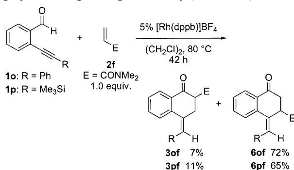
Scheme 10. Rhodium-catalyzed regioselective [4+2] carbocyclization of 2-alkynylbenzaldehydes with N,N -dimethylacrylamide.
