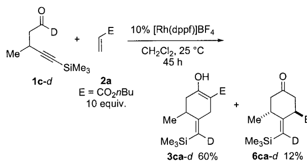
Scheme 13. Deuterium labeling study.
