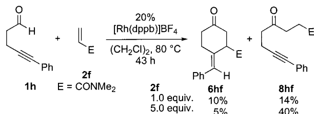
Scheme 14. Rhodium-catalyzed reaction of 5-phenyl-4-pentynal with excess N,N -dimethylacrylamide.
