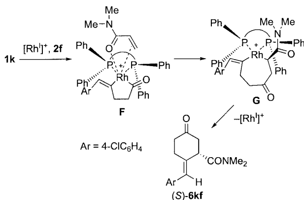
Scheme 15. Possible mechanism of the selective formation of ( S )- 6kf .
