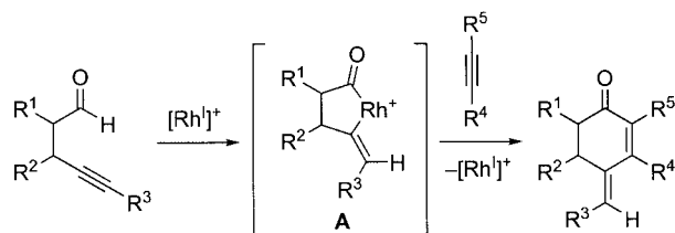
Scheme 1. Rhodium-catalyzed intermolecular [4+2] carbocyclization of 4-alkynals with alkynes leading to cyclohexenones.
