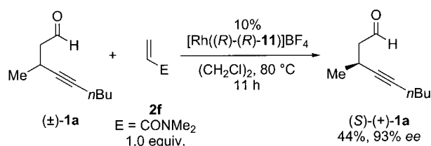
Scheme 9. Rhodium-catalyzed enantioselective kinetic resolution of 3-methyl-4-nonynal.
