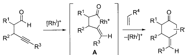
Scheme 2. Rhodium-catalyzed intermolecular [4+2] carbocyclization of 4-alkynals with alkenes leading to cyclohexanones.
