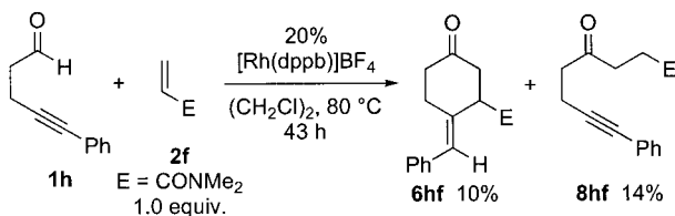
Scheme 7. Rhodium-catalyzed regioselective [4+2] carbocyclization of 5-phenyl-4-pentynal with N,N -dimethylacrylamide.
